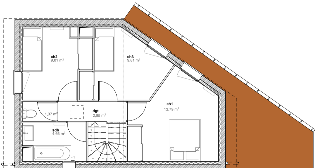
PLAN R+1
